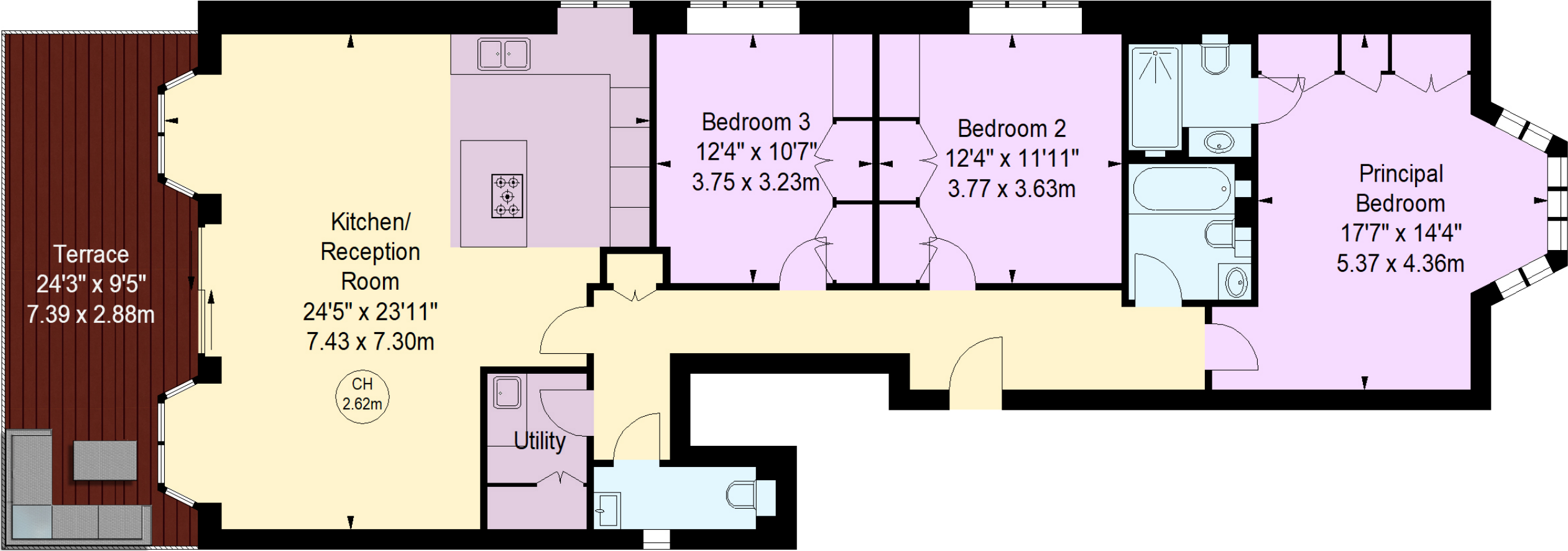
GROUND FLOOR
