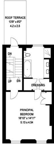
FIRST FLOOR
